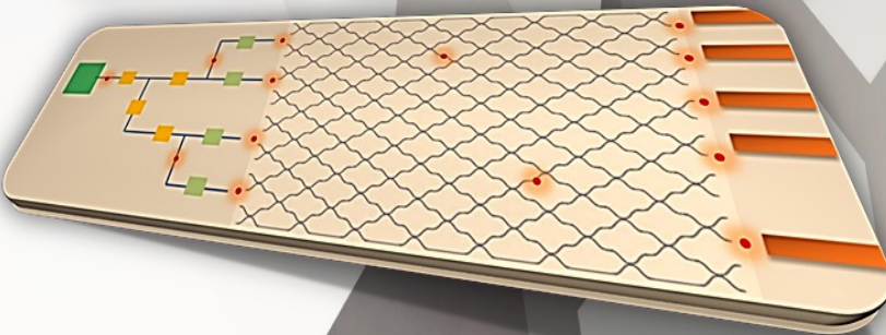
Photonic Quantum Processor.
